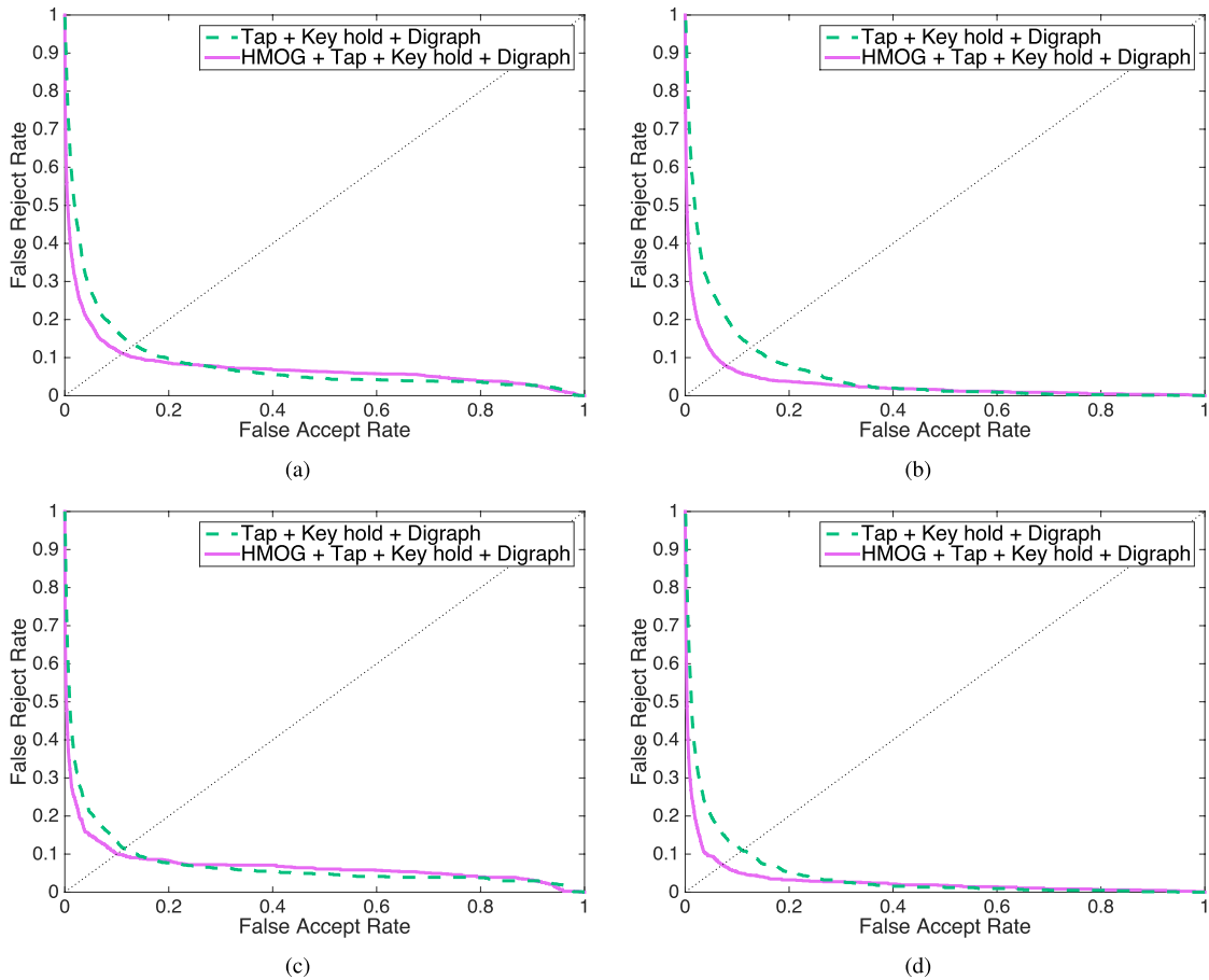
Fig. 7. DET curves for fusion of all feature types including and excluding HMOG. The scan lengths are 60- and 120-second scans. (a) Sitting (60-second scans). (b) Walking (60-second scans). (c) Sitting (120-second scans). (d) Walking (120-second scans).
