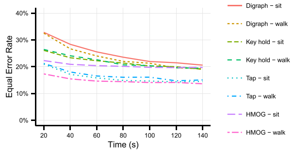
Fig. 5. Comparison of EERs of HMOG with keystroke dynamics (i.e., key hold and digraph) and tap features with SM verifier. X-axis shows authentication time in seconds.
